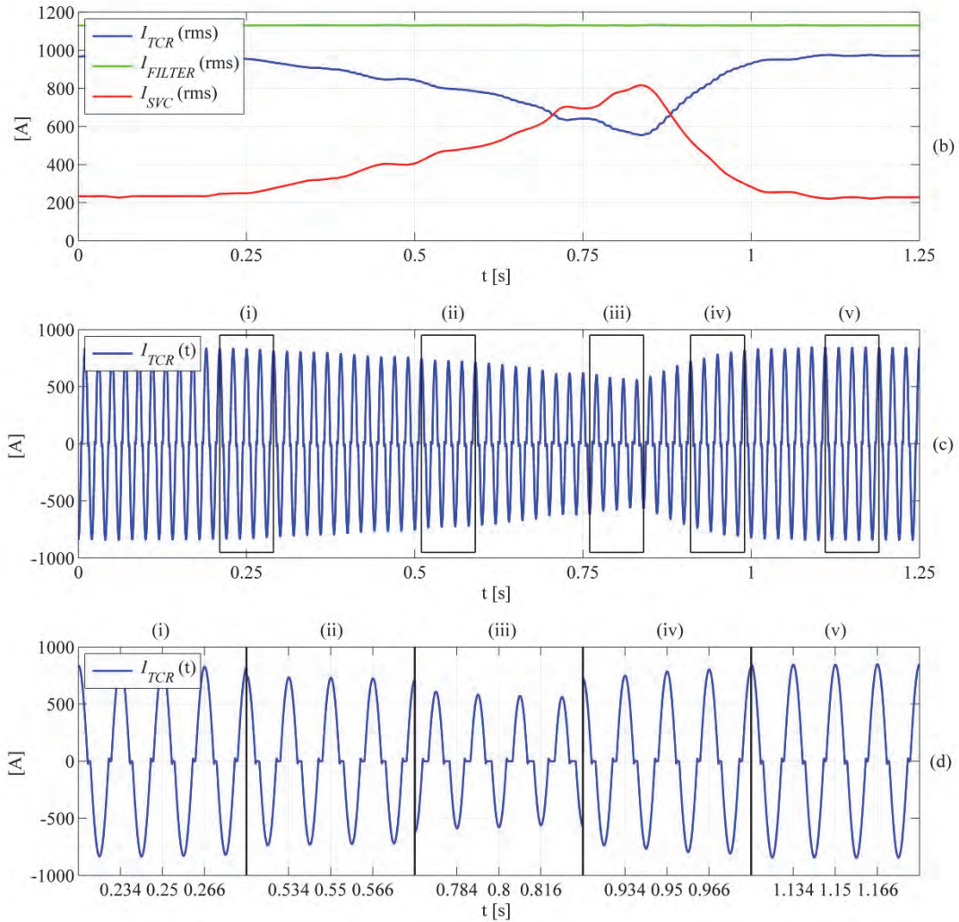
Fig. 8: Simulated SVC currents
