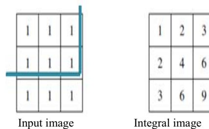
Fig. 7. Integral image computation
