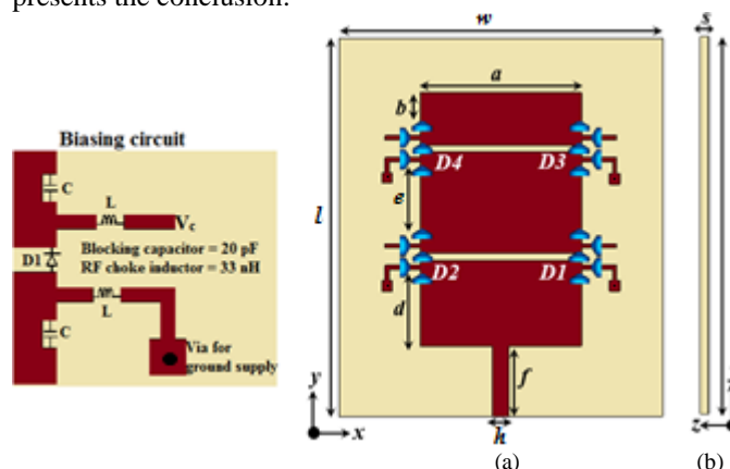
Fig.1:Proposed frequency and pattern reconfigurable antenna(a)Front view l=50\text{mm} , w=50\text{mm} , f=13\text{mm} , h=3\text{mm} , a=30\text{mm} , b=9\text{mm} , e=17\text{mm} , d=15\text{mm} , s=1.6\text{mm} (Black dot represents the via). (b) Side view.
