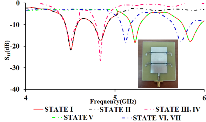
Fig 3: Measured reflection coefficient characteristics of the proposed antenna (Photograph of the fabricated prototype is shown as an inset)
